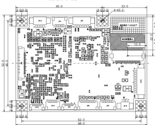
MAIN-PCB
