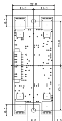
POWER-PCB
